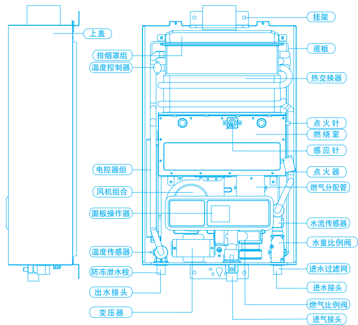
a. JSQ48-Hi7/JSQ48-Hi7S/JSQ40-Hi7/JSQ40-Hi7S机型:
