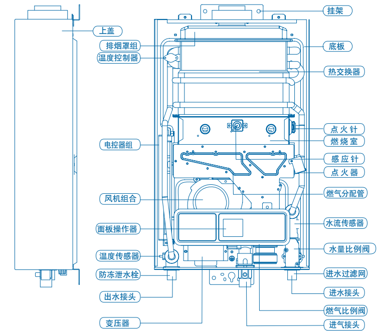
c. JSG32-Hi7/JSG32-Hi7S机型:
