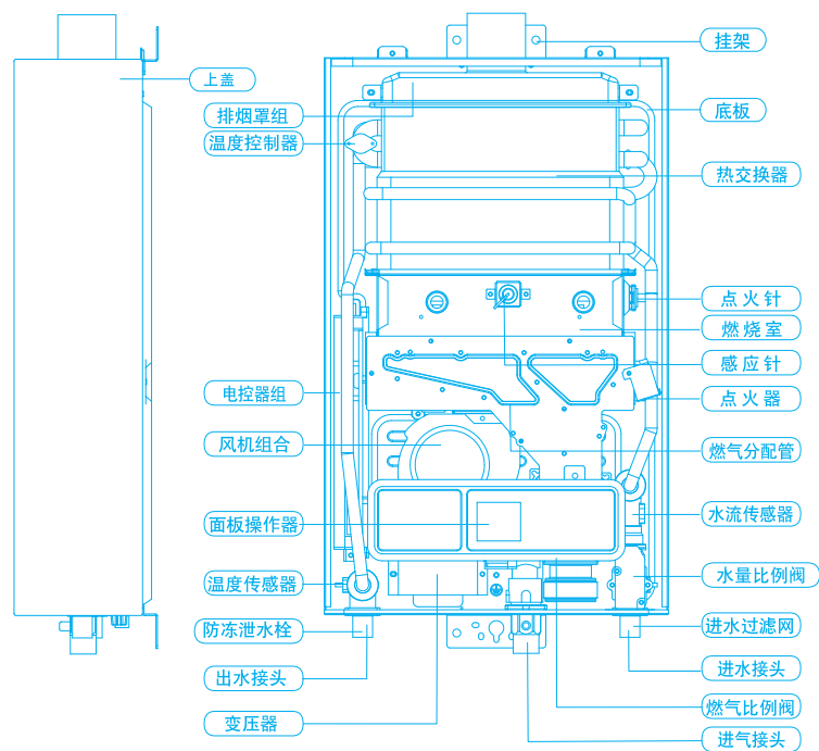
b. JSQ32-Hi7/JSQ32-Hi7S/JSQ26-Hi7/JSQ26-Hi7S机型:
